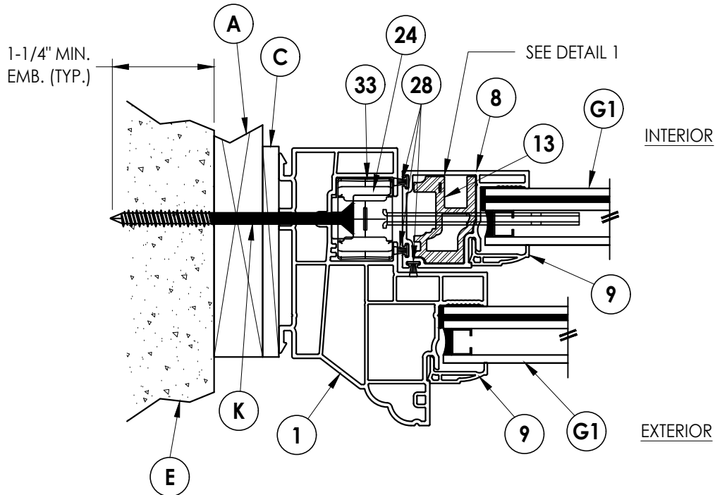
3 HORIZONTAL CROSS SECTION Shown w/ 1X Buck
