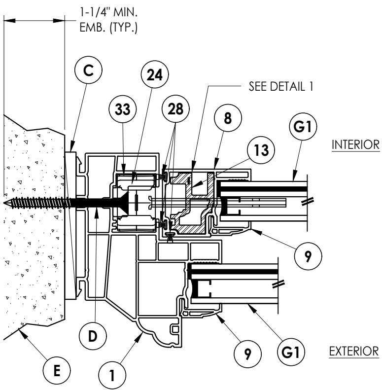
2 HORIZONTAL CROSS SECTION Shown Direct to Masonry
